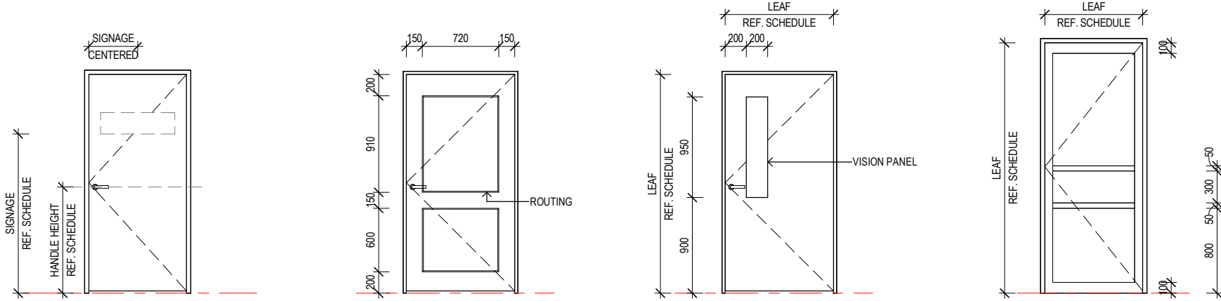
DOOR DIMENSION DIAGRAM APPLIES TO LEAF TYPES A18, C2,4, P5-11
